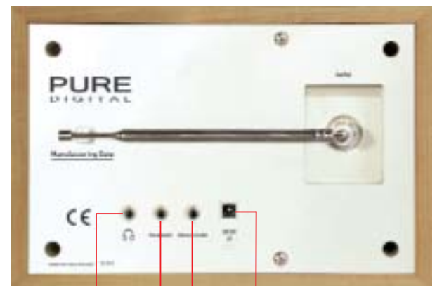
Headphone Socket Auxiliary Speaker Output Power Input Stereo Line Out to Hi-Fi or Recorder
