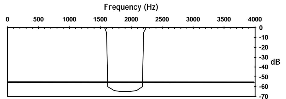
Typical Band-stop Filter Response
