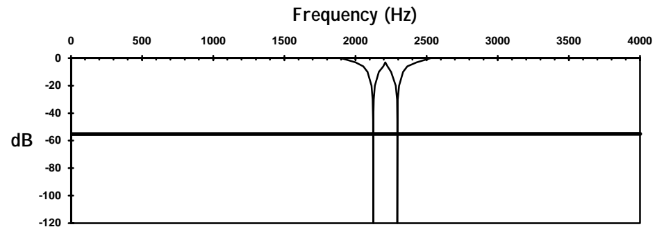
Typical Manual Notch Filter Response
