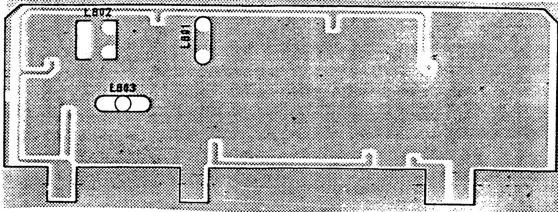
8801 PH-144AA 800 MHZ PCB TOP VIEW
